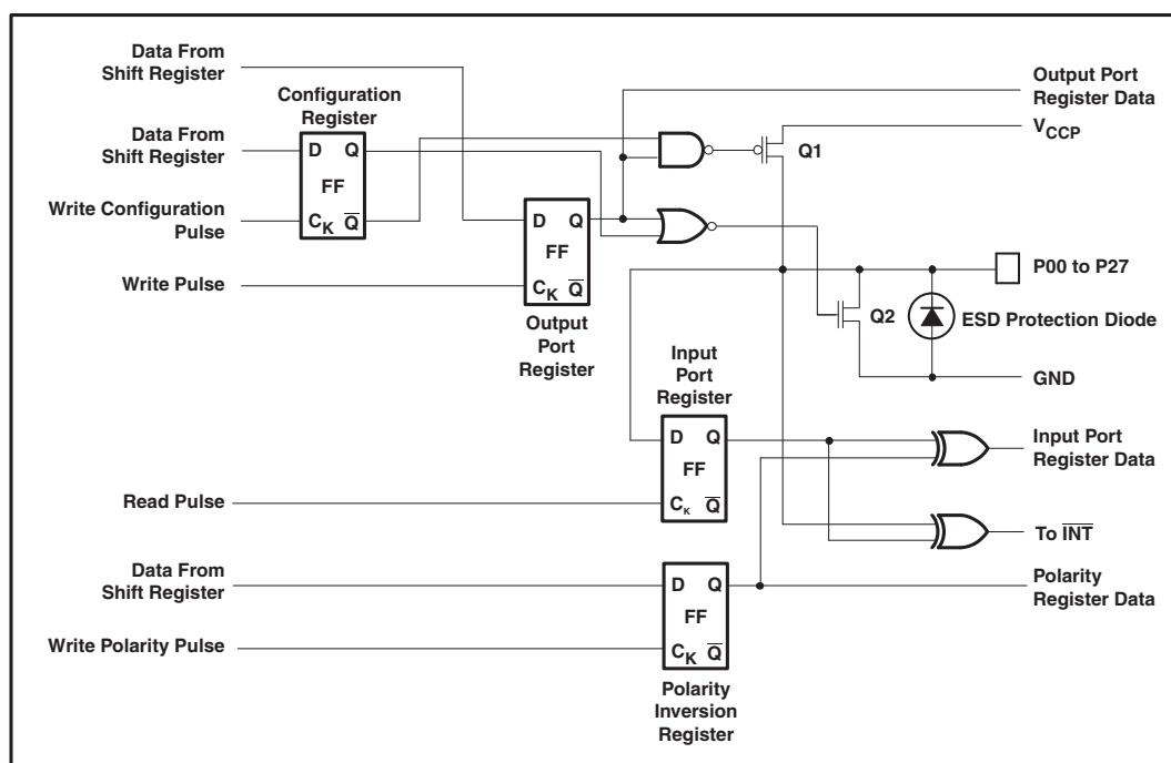
Simplified Schematic of P00 to P27
