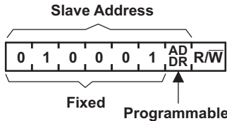
Figure 4. TCA6424 Address
