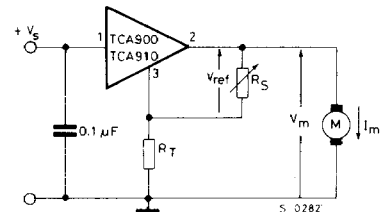
Fig. 2 - Typical application circuit.
