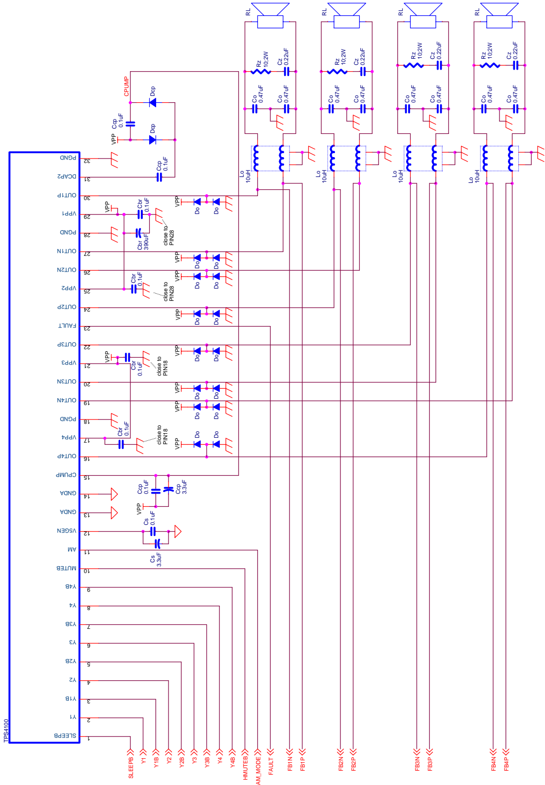
TPS4100 Connection Diagram
