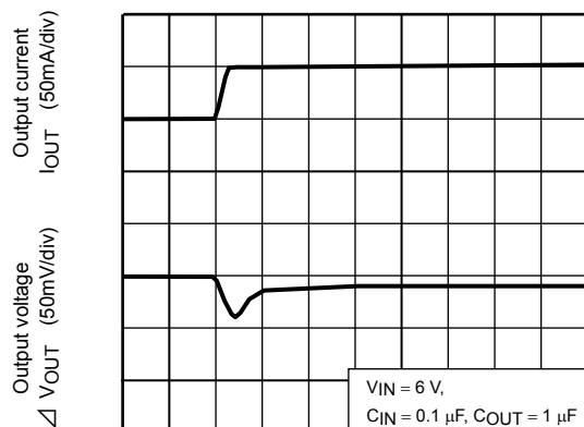
TCR5SB50 ( I_{OUT} = 50\text{m to } 100\text{mA} )
