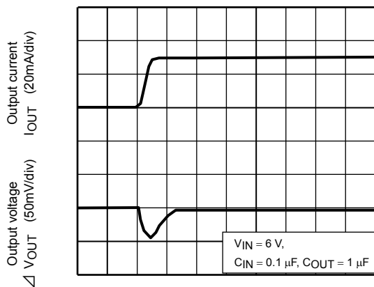
TCR5SB50 ( I_{OUT} = 1\text{m to } 30\text{mA} )
