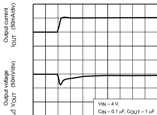
TCR5SB30 ( I_{OUT} = 50\text{m to } 100\text{mA} )
