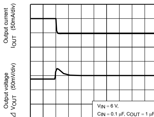
TCR5SB50 ( I_{OUT} = 100\text{m to } 50\text{mA} )
