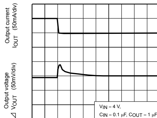
TCR5SB30 ( I_{OUT} = 100\text{m to } 50\text{mA} )
