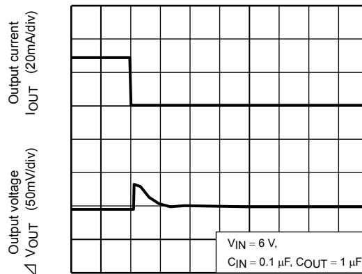
TCR5SB50 ( I_{OUT} = 30\text{m to } 1\text{mA} )
