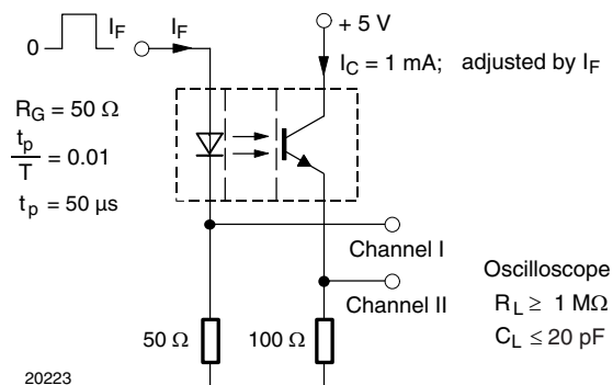
Figure 1. Test Circuit for t_{on} and t_{off}
