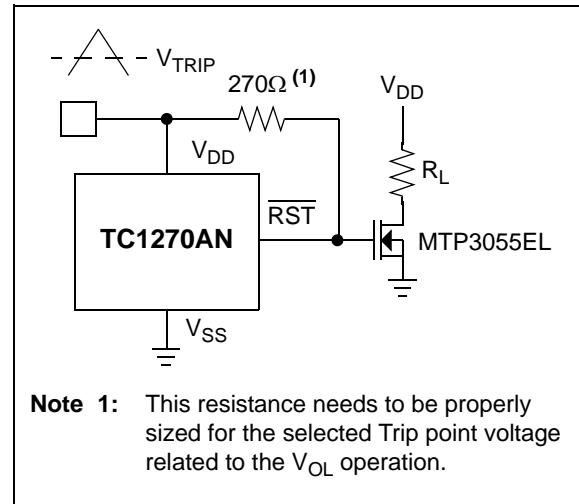
FIGURE 5-6: MOSFET Low-Drive Protection.
