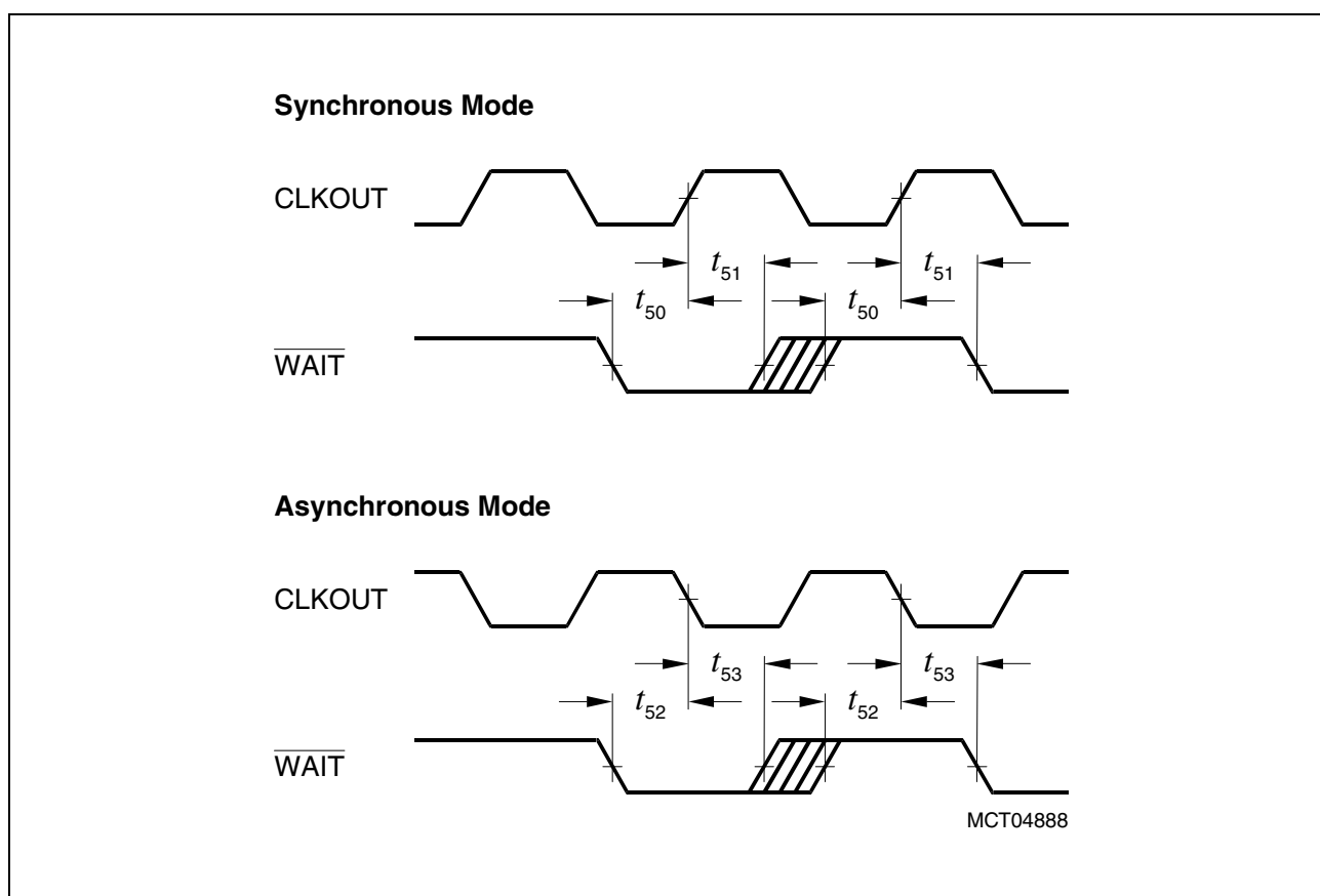
Figure 36 \overline{\text{WAIT}} Timing (from FPI Bus to external Memory)
