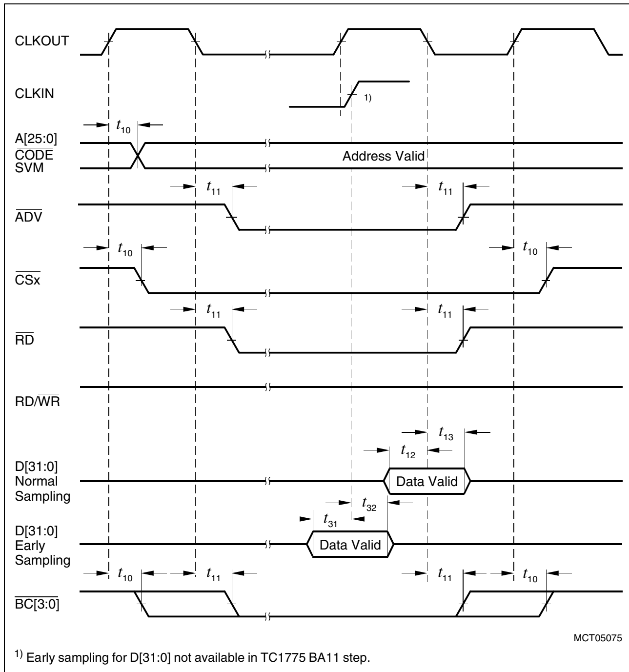
Figure 32 EBU Demultiplexed Read Timing
