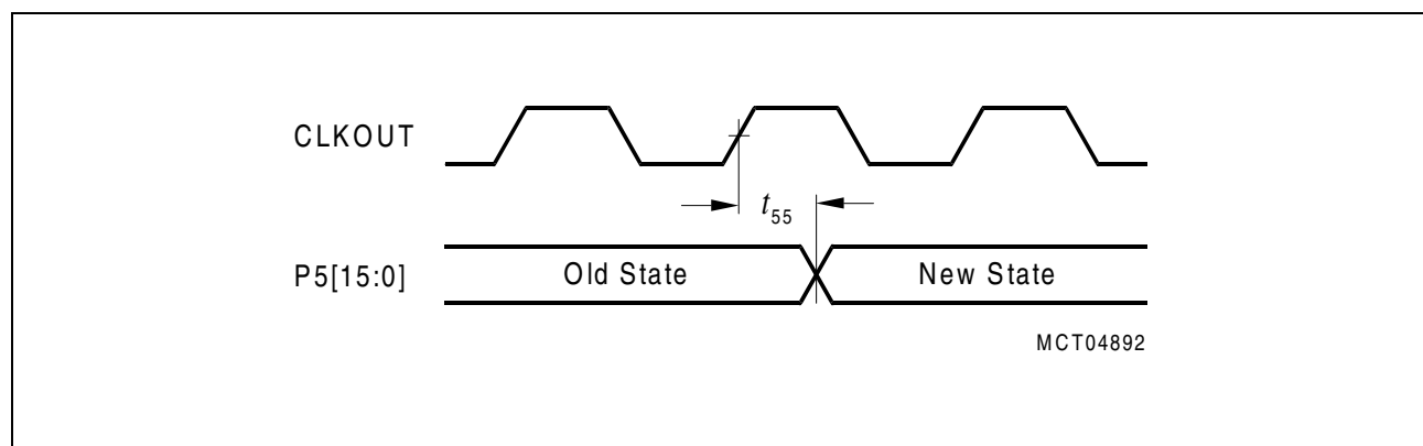
Figure 40 Port 5 Timing
