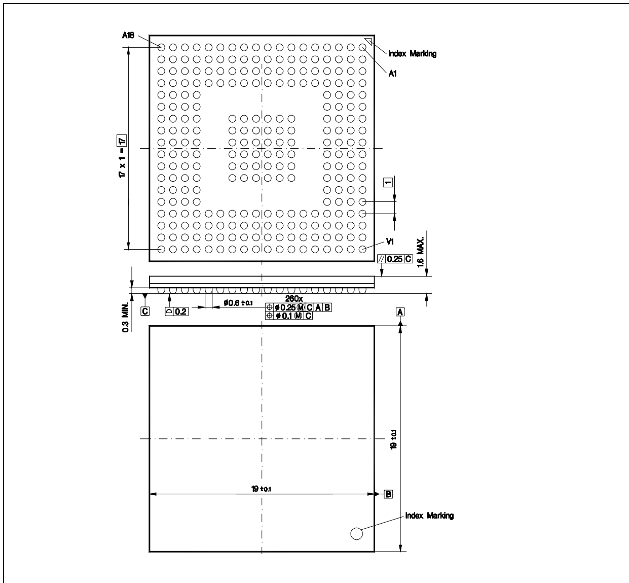
Figure 31 LBGA-260 Package
