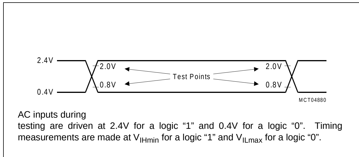
Figure 18 Input/Output Waveforms for AC Tests - for GPIO, Dedicated and EBU pins
