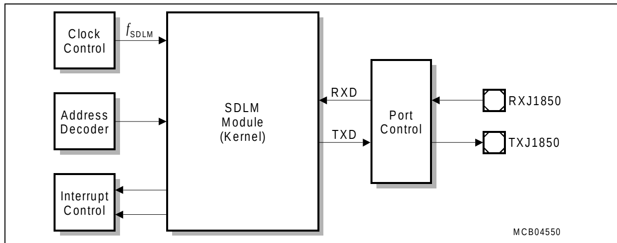
Figure 11 General Block Diagram of the SDLM Interface
