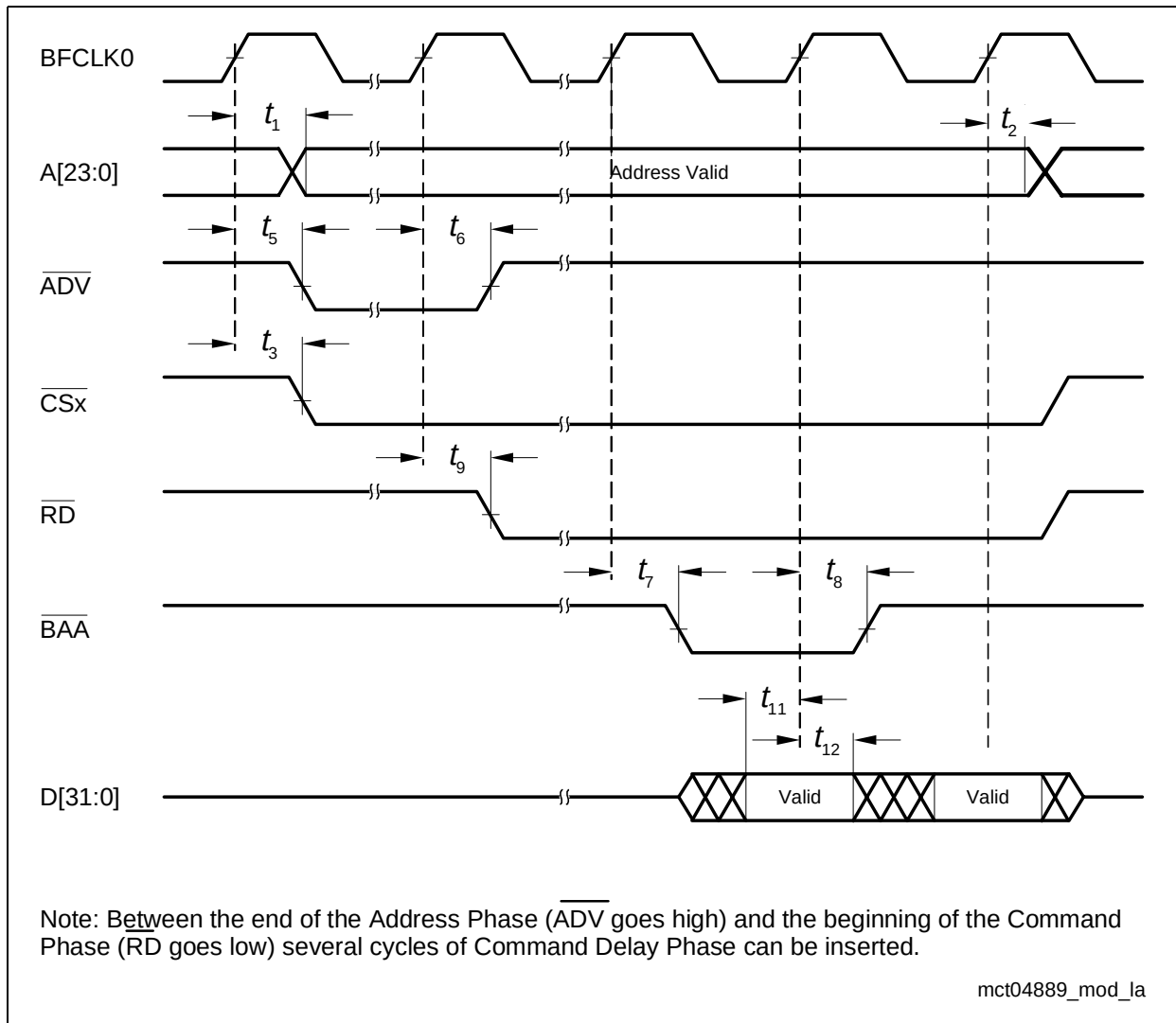
Figure 24 Burst Flash Access Timing (Instruction Read)
