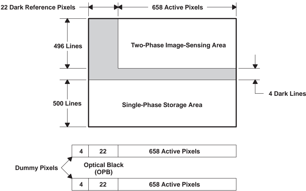
sensor topology diagram
