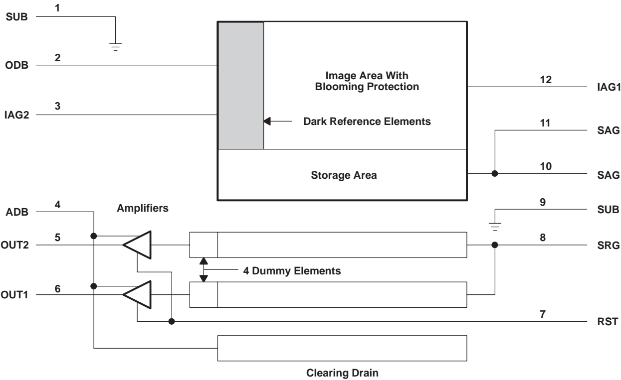
sensor topology diagram
