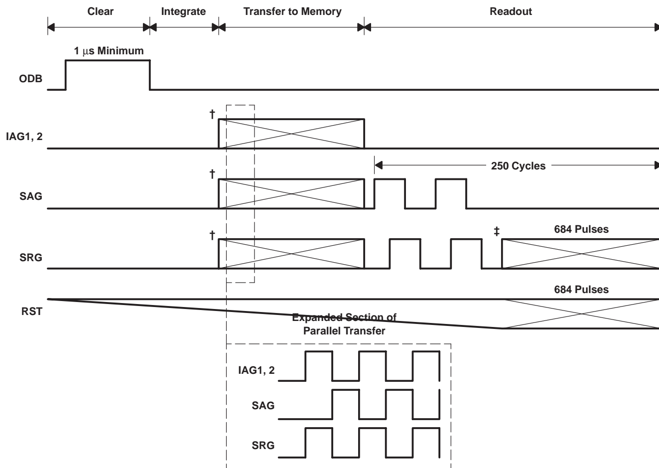
Figure 4. Interlace Timing
