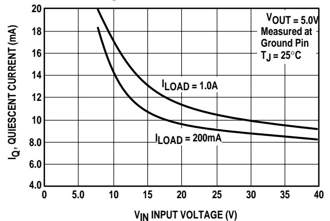
Figure 25. Quiescent Current
