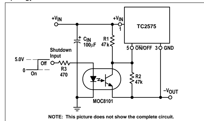
Figure 10. Inverting Buck-Boost Regulator Shutdown
