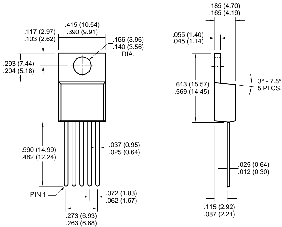
5-Pin TO-220
