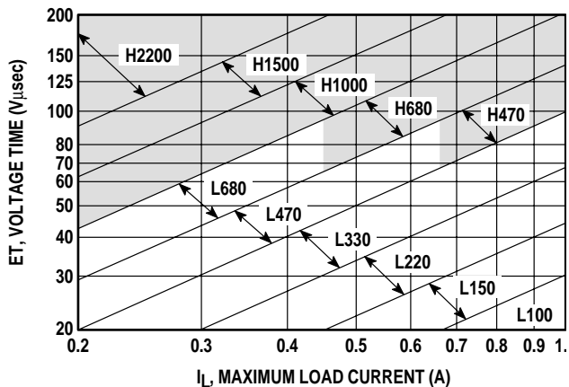
Figure 35. TC2575-Adj
