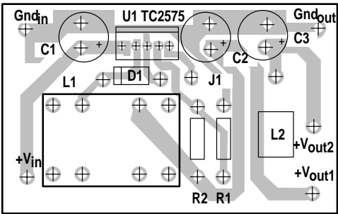
Figure 18. PC Board Component Side
