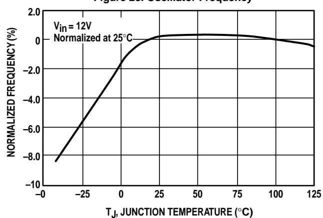
Figure 28. Oscillator Frequency
