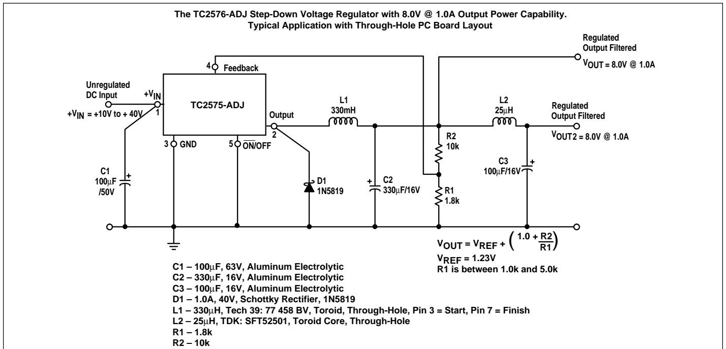
Figure 17. Schematic Diagram of the 8.0V at 1.0A Step-Down Converter Using the TC2575-ADJ
