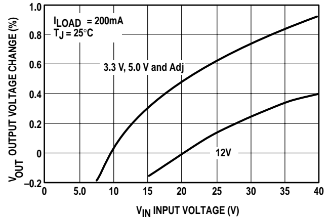
Figure 21. Line Regulation
