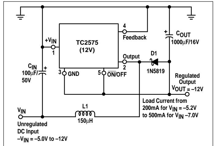
Figure 12. Negative Boost Regulator
