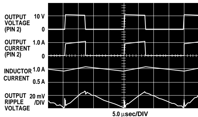
Figure 30. Switching Waveforms
