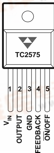
5-Pin TO-220
