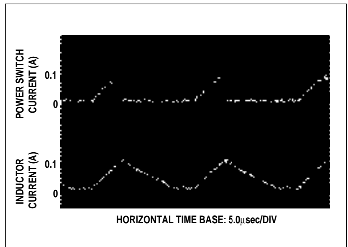
Figure 6. Discontinuous Mode Switching Current Waveforms
