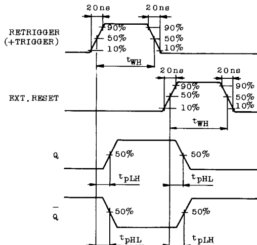
WAVEFORM 3.
