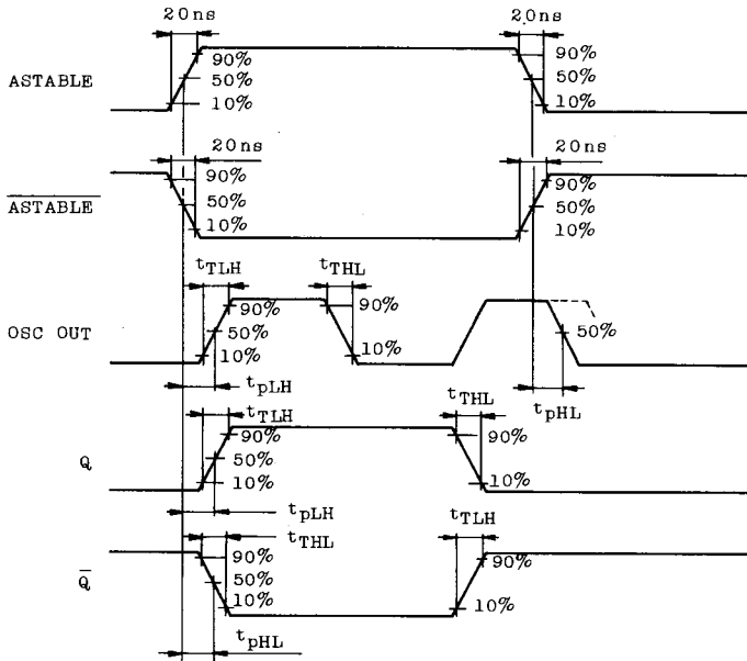
WAVEFORM 2.
