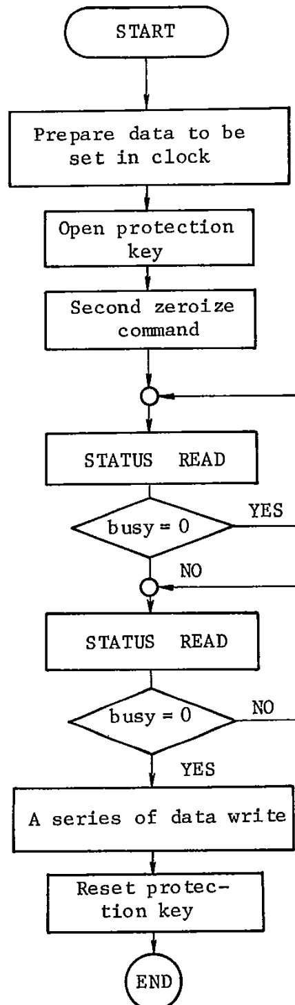
Fig. 5.5 Program Flow (3)
