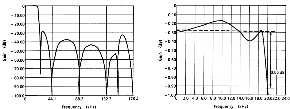
Figure 3 Digital Filter Frequency Characteristics ( f_s = 44.1\text{ kHz} )
