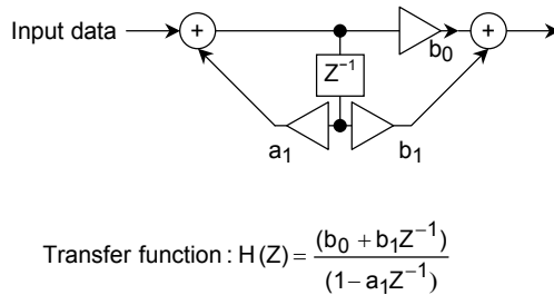
Figure 4 IIR Digital De-Emphasis Filter
