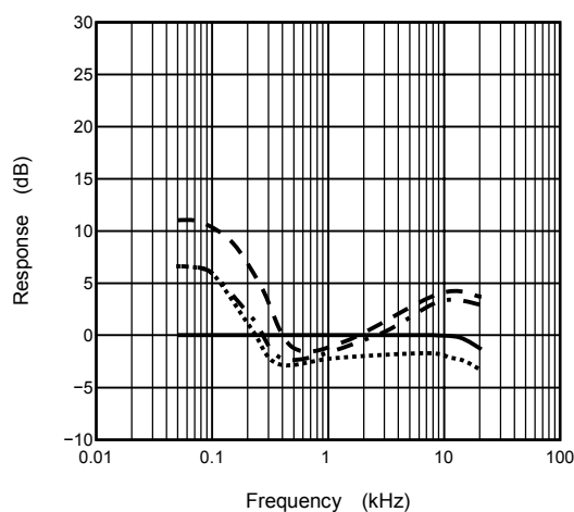
b) V_{in} = -20\text{dB} input, DBB OFF, 1 kHz = 0dB.
