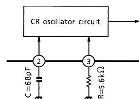
Figure 1 CR Oscillator circuit
