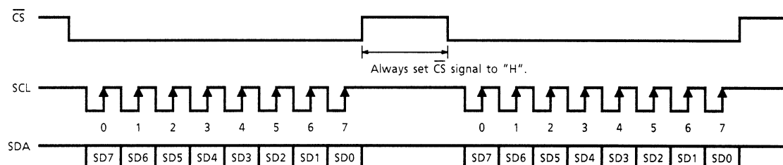
Figure 4 Serial control timing
