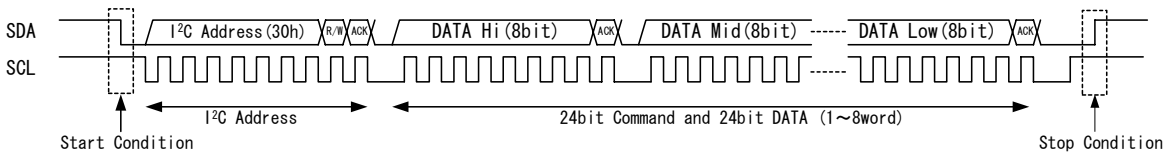
Figure 10 Data Transmission Format in I 2 C Mode
