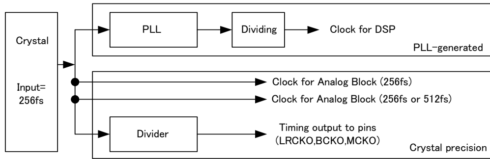
Figure 1 Timing System
