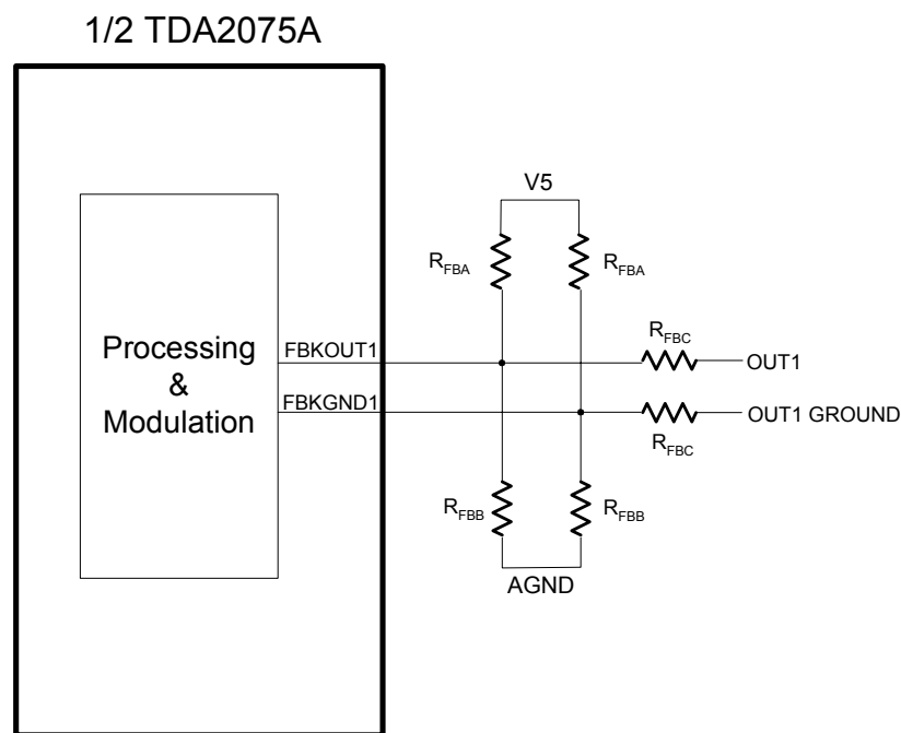
Figure 3: Modulator Feedback
