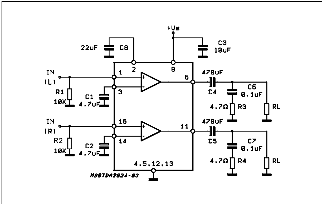
Figure 1 : Test Circuit (stereo).
