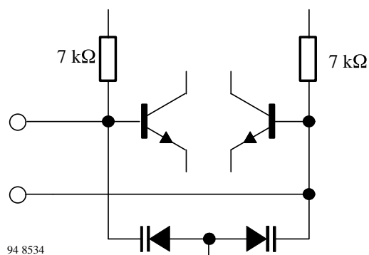
Figure 18. VCO (Pin 20-21)
