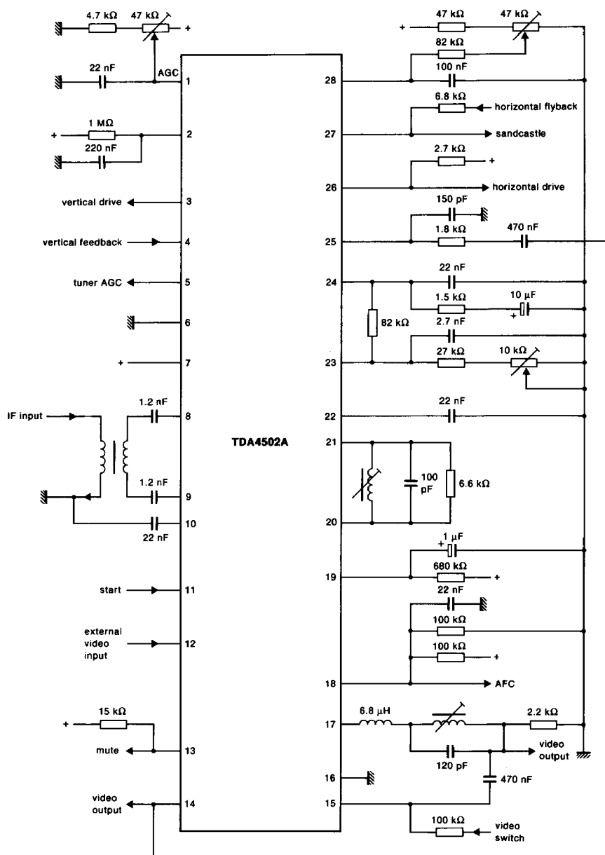
Fig. 8 Application diagram.
