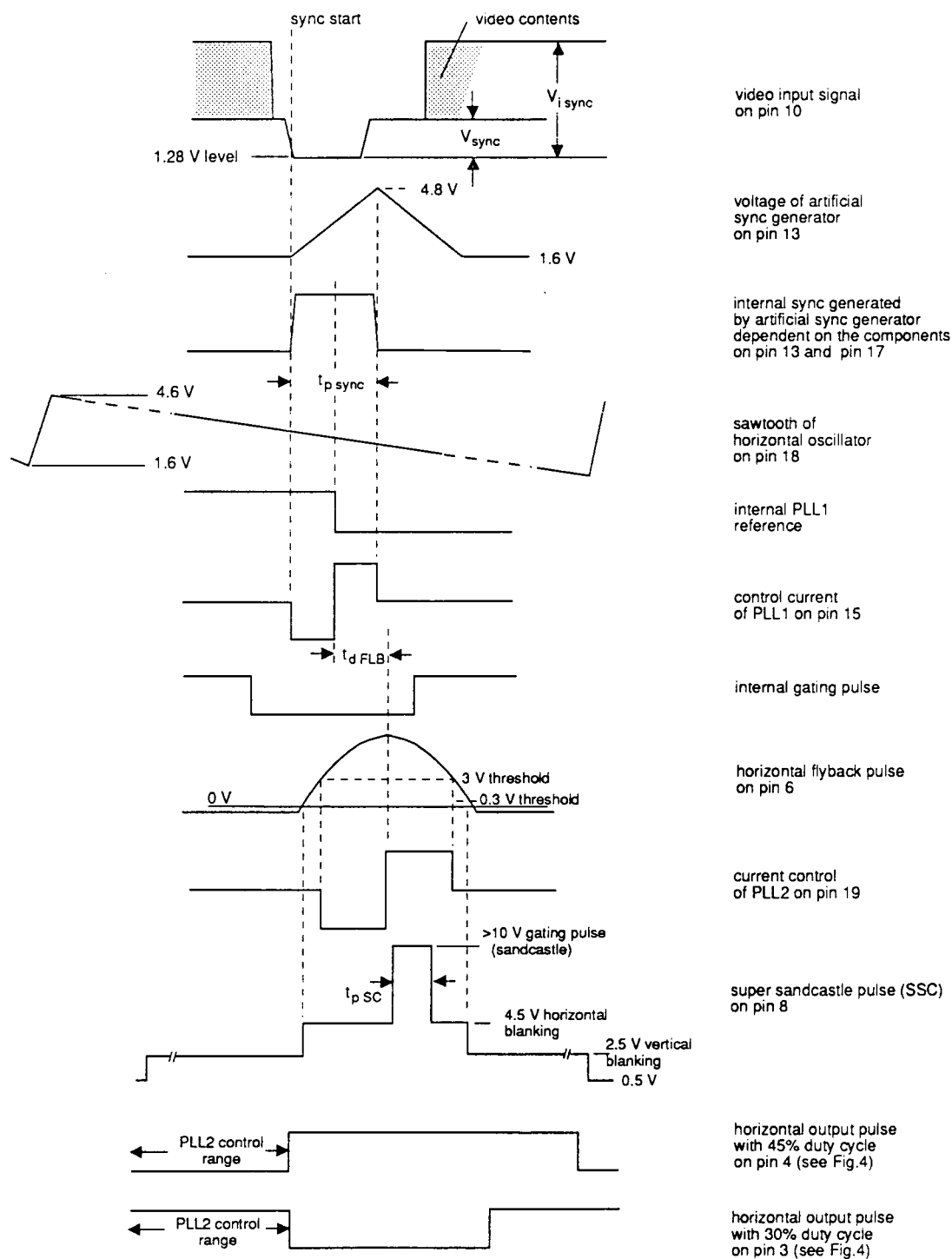
Fig.6 Timing diagram using the artificial sync generator.
