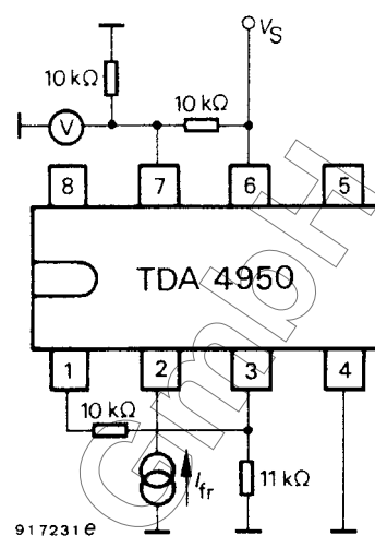
Figure 5. Test circuit 2
