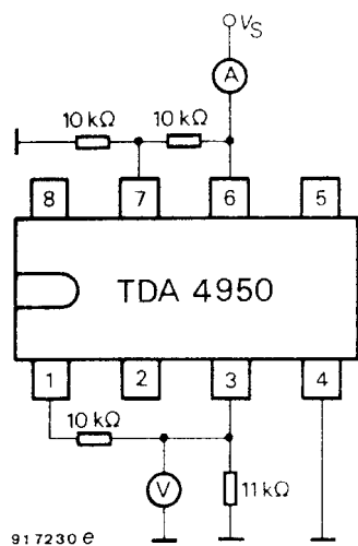
Figure 3. Test circuit 1
