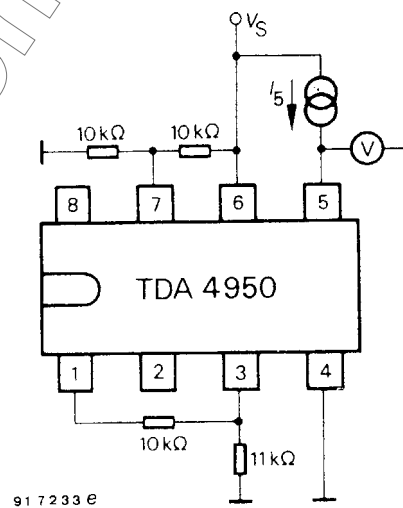
Figure 6. Test circuit 4
