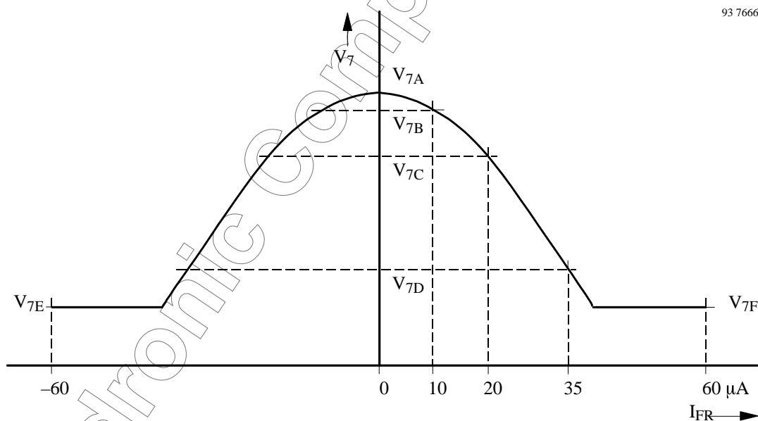
Figure 2. Parabola coefficients
