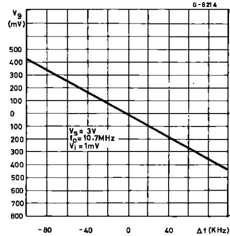
Figure 16 : AFC Output Voltage (Pin 9) versus Frequency Deviation (FM section)
