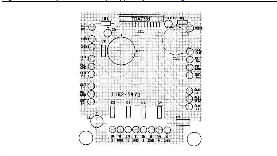
Figure 4. Components and top copper layer of the Figure 3
