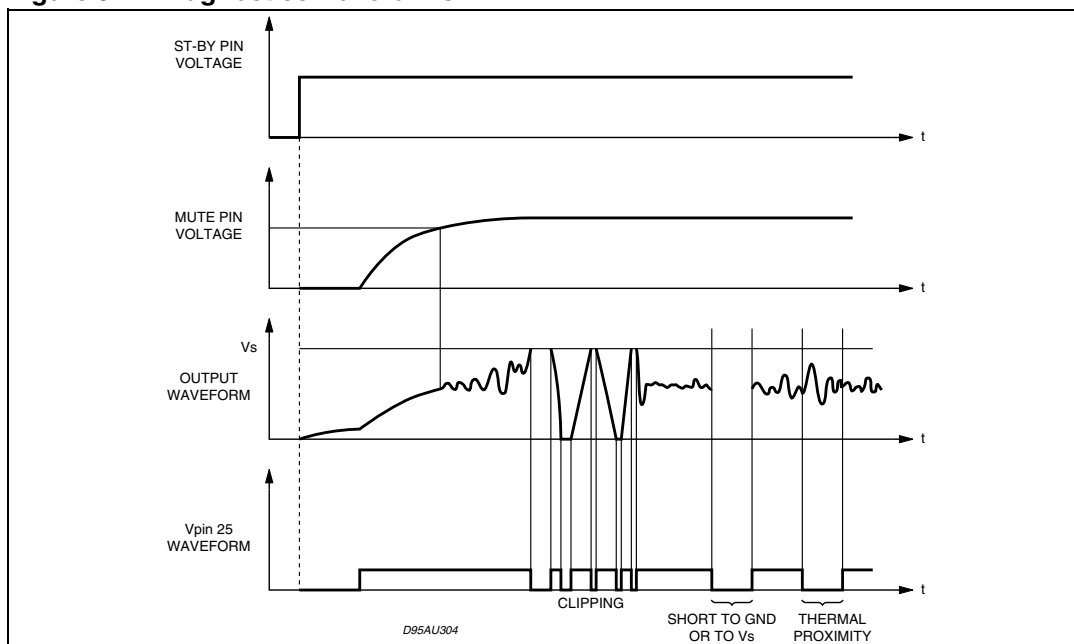
Figure 9. Diagnostics waveforms
