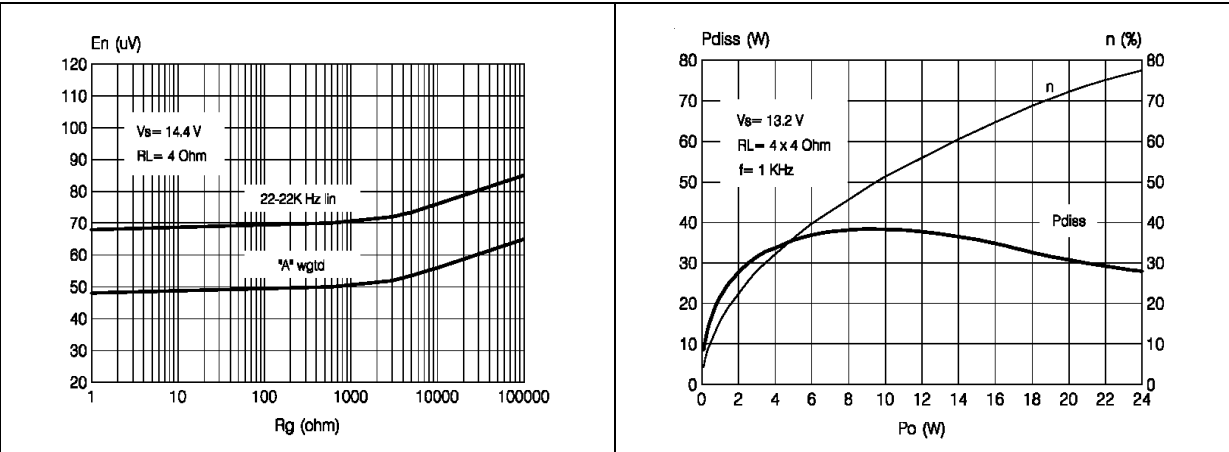
Figure 15. Power dissipation and efficiency vs. output power
