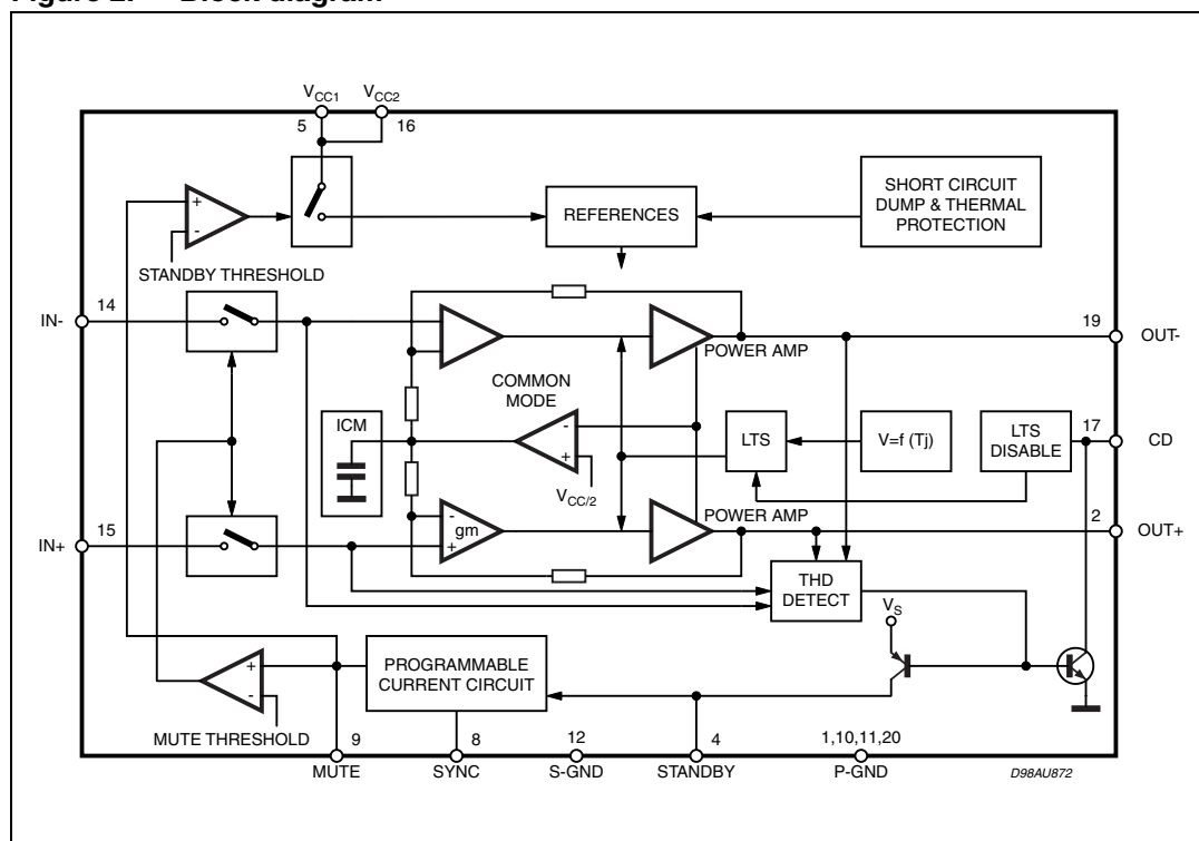
Figure 2. Block diagram
