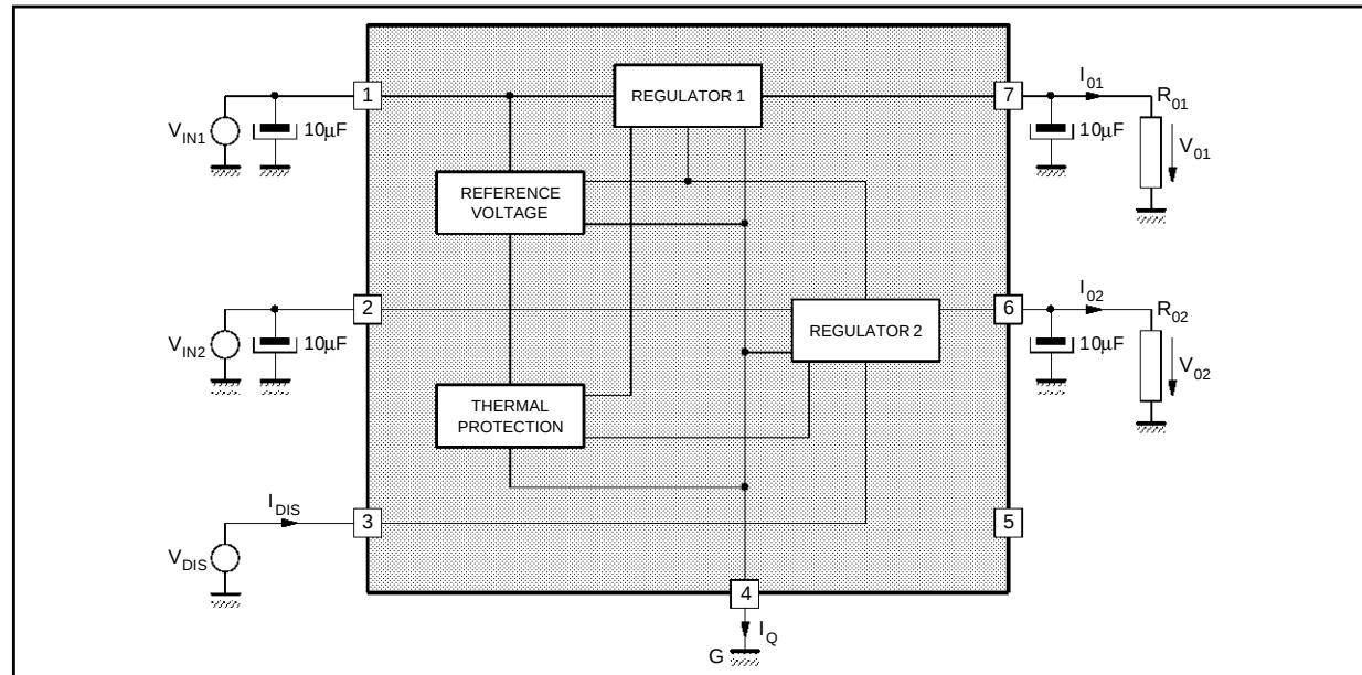
Figure 1 : Test Circuit
