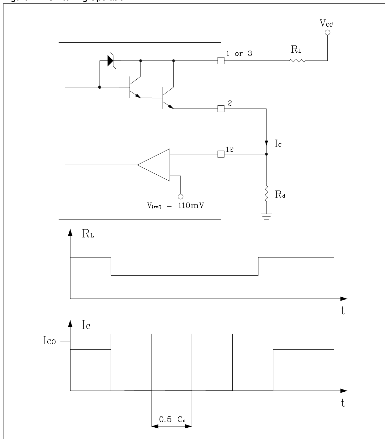
Figure 2. Switching Operation
