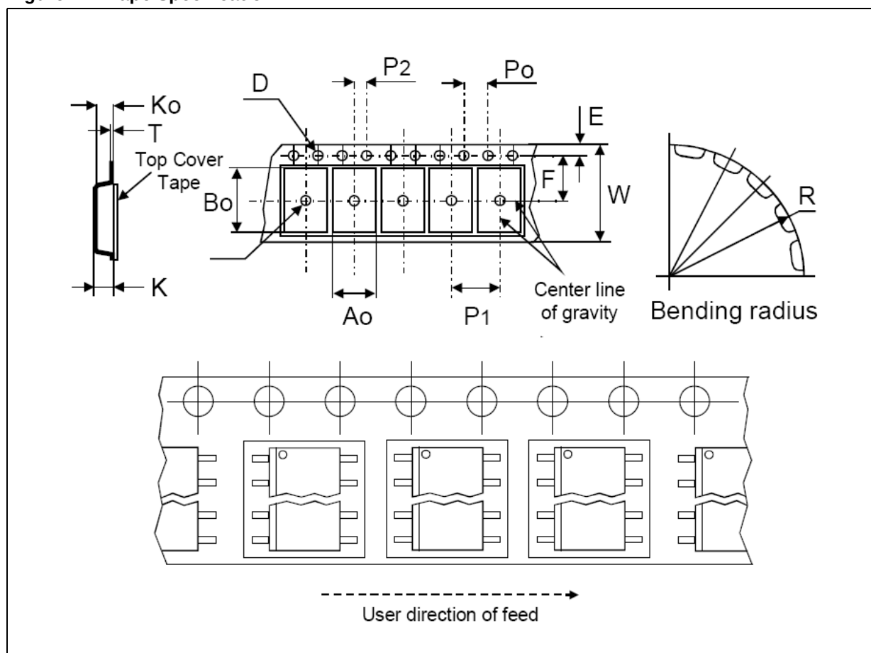
Figure 14. Tape Specification
