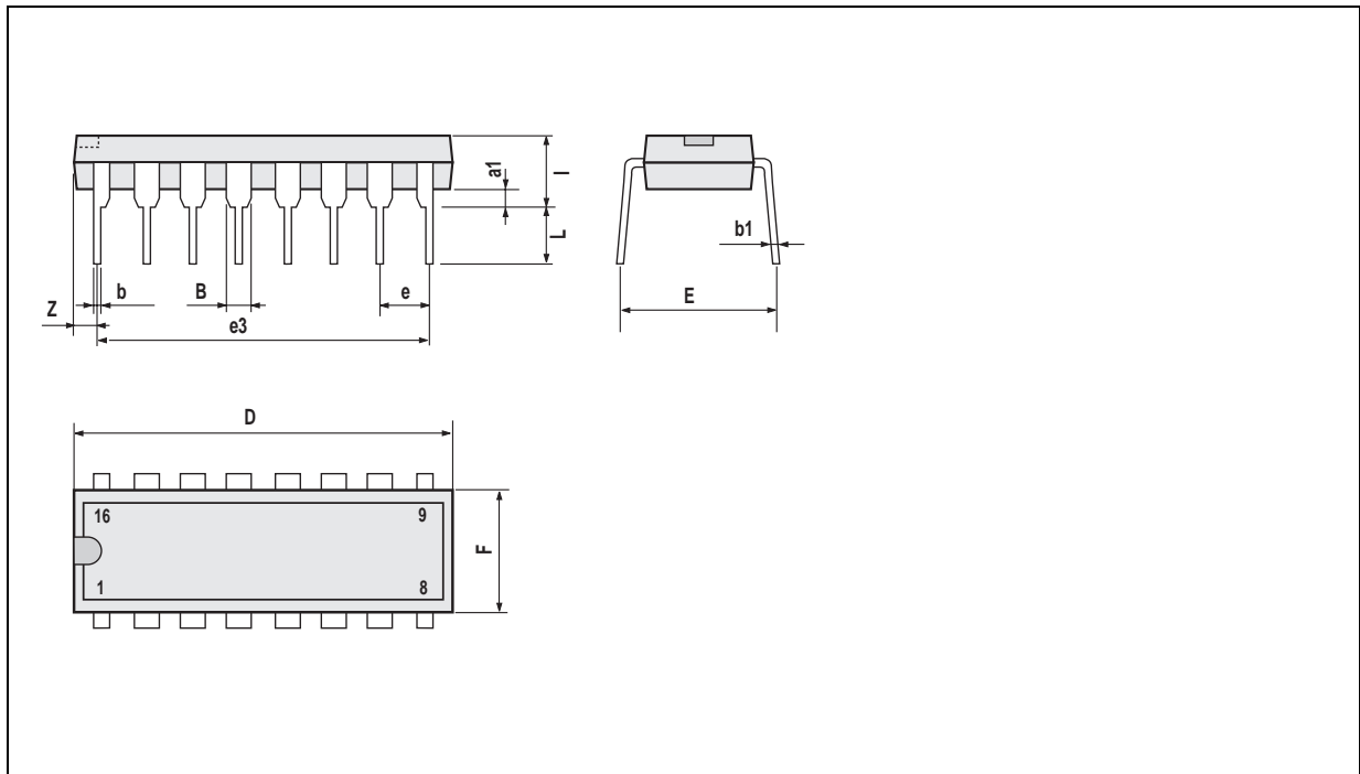
Figure 7. 16-Pin Package
