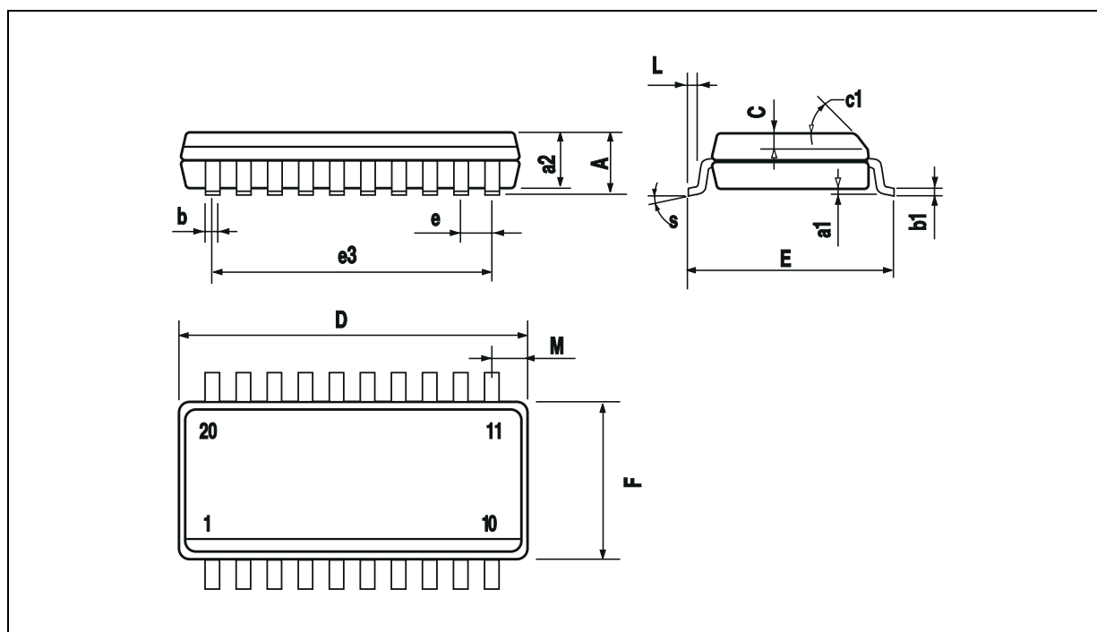
Figure 11. 20-Pin Package
