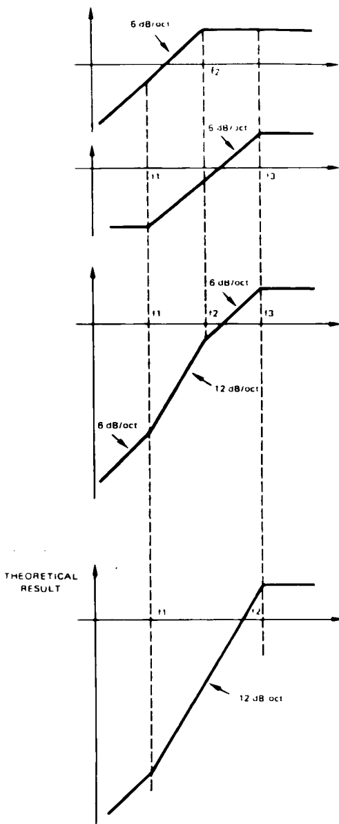
Figure 16 : Antilarsen System Filter Response.
