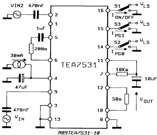
Figure 7 : Loudspeaker Amplifier : Gain/Distortion/Output Offset.
