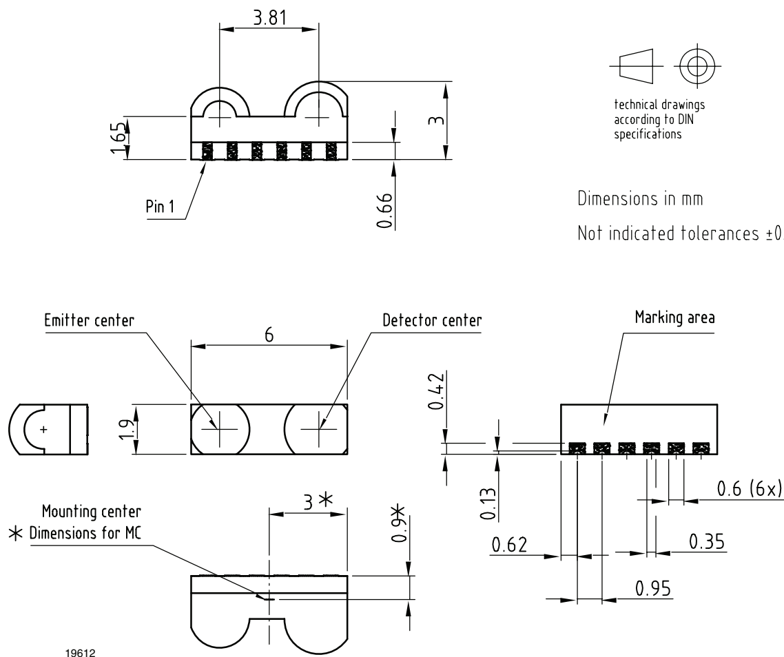
Figure 4. Package drawing of TFBS4711, tolerance of height is + 0.1mm, - 0.2 mm, other tolerances \pm 0.2 mm
