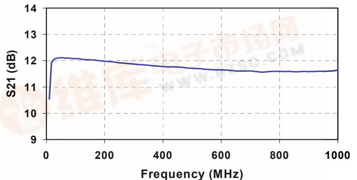
Gain in a Typical Circuit w/External Balun Effects Removed
