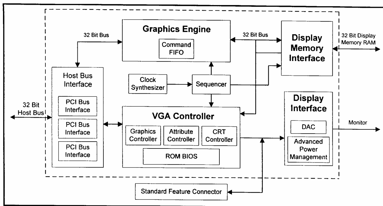
TGUI9440-R Block Diagram
