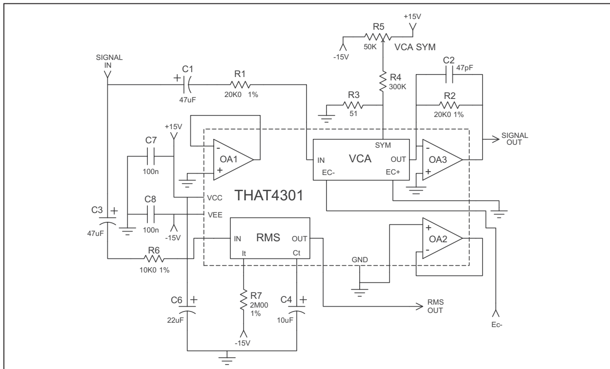
Figure 2. VCA and RMS detector test circuit
