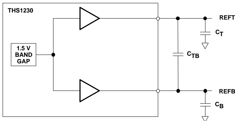
Figure 1. Reference Generation
