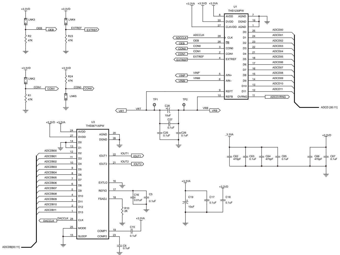
Figure 22. EVM Schematic
