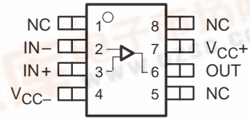
THS4081 D OR DGN PACKAGE (TOP VIEW)
