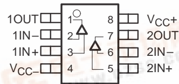
THS4082 D OR DGN PACKAGE (TOP VIEW)
