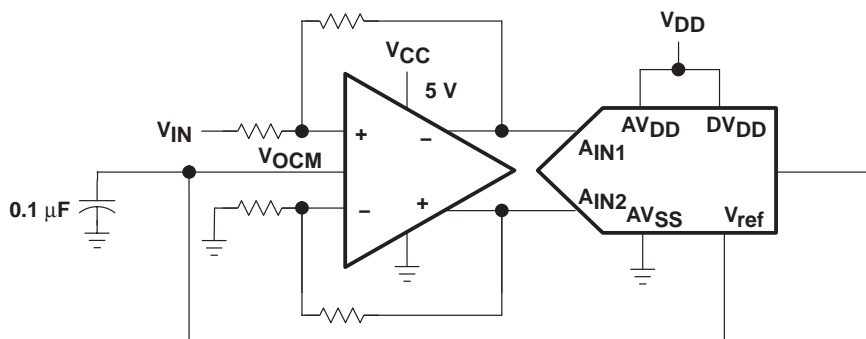
Figure 31. Fully Differential Amplifier Using a Single Supply
