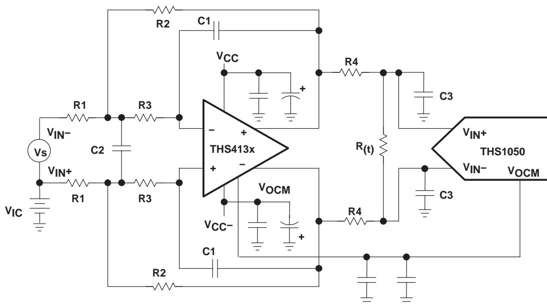
Figure 34. Antialias Filtering
