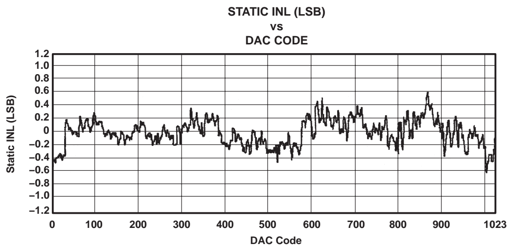
Figure 8. Static INL
