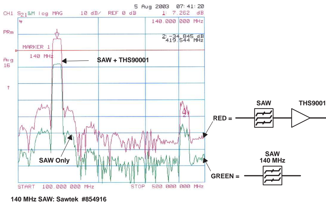
Figure 24. Frequency Response of the THS9001 and SAW Filter, and SAW Filter Only
