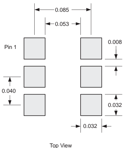
Figure 28. THS9001 Recommended Footprint (dimensions in inches)
