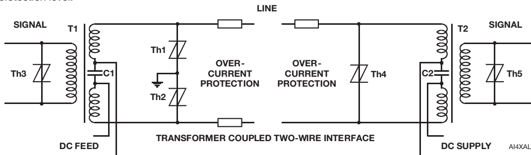
Figure 11. 2-Wire System
