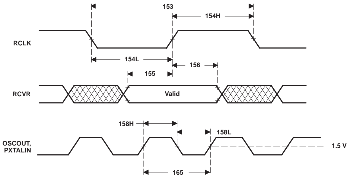
Figure 12. Ring-Interface Timing
