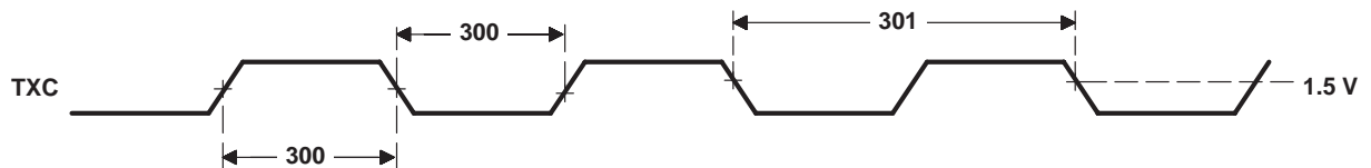
Figure 14. Ethernet Timing of TXC
