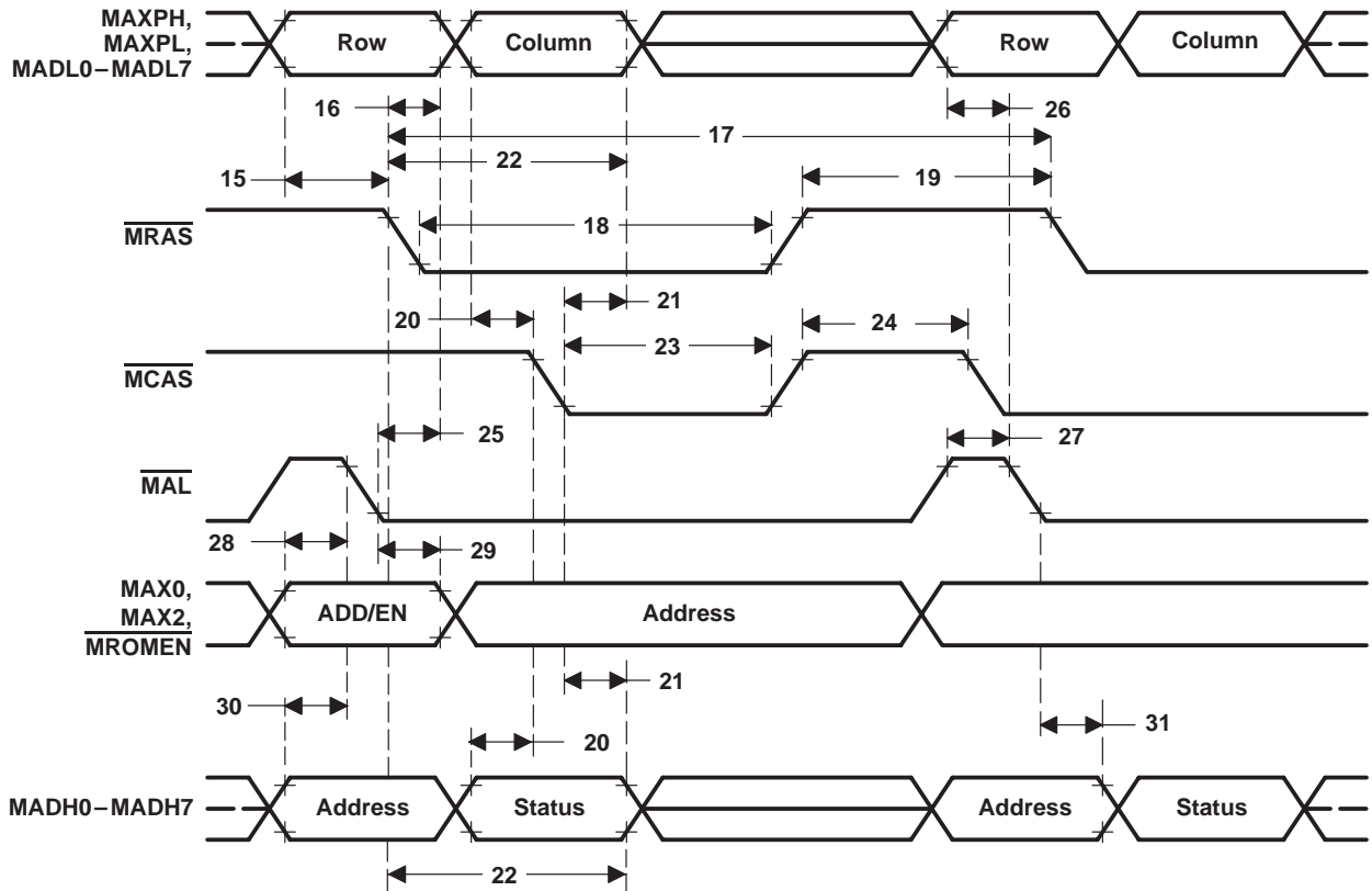
Figure 7. Memory-Bus Timing: Clocks, \overline{MRAS} , \overline{MCAS} , and \overline{MAL} to ADDRESS
