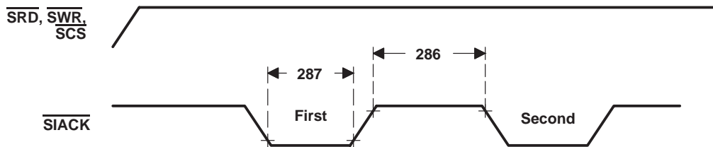
Figure 23. 80x8x Interrupt-Acknowledge-Cycle Timing: First \overline{\text{SIACK}} Pulse
