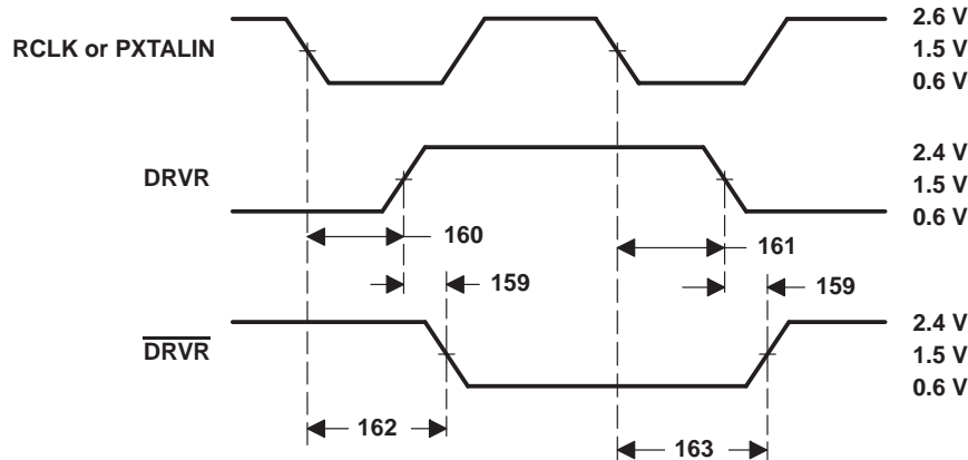
Figure 13. Skew and Asymmetry From RCLK or PXTALIN to \overline{DRVR} and DRVR
