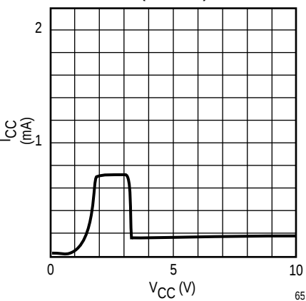
INPUT CURRENT vs. INPUT VOLTAGE (NO LOAD)
