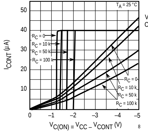
CONTROL CURRENT vs. CONTROL VOLTAGE
