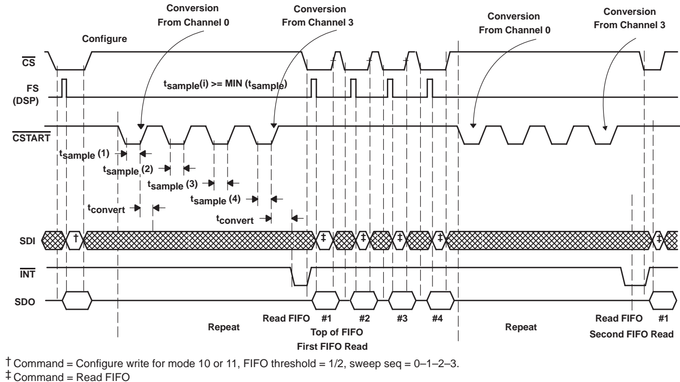
Figure 13. TLC1514/TLC1518 Mode 10/11 DSP Serial Interface (conversions triggered by \overline{CSTART} )
