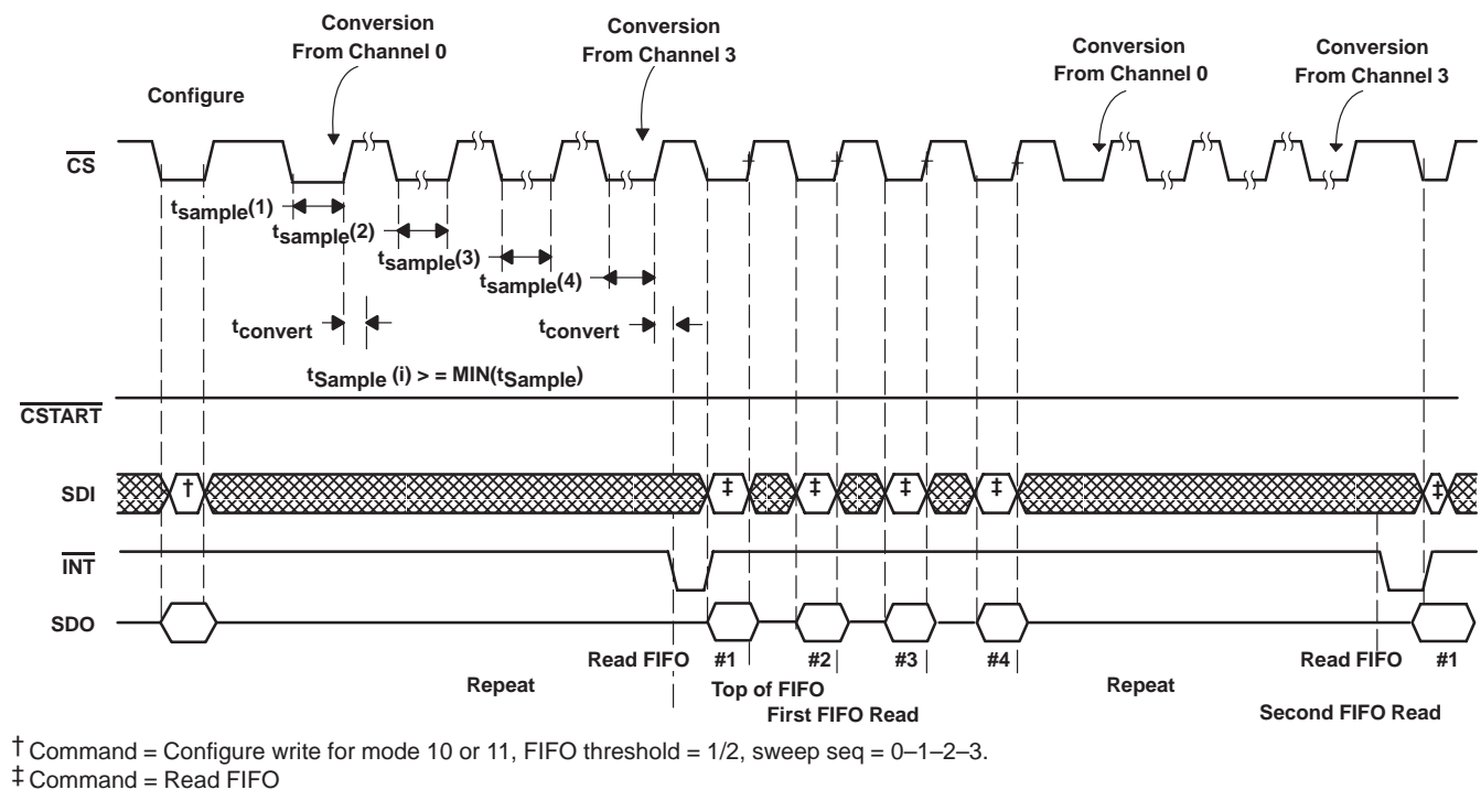
Figure 14. TLC1514/TLC1518 Mode 10/11 \mu p Serial Interface (conversions triggered by \overline{CS} )
