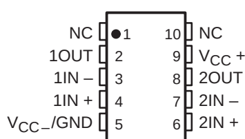
TLC2262M, TLC2252AM . . . U PACKAGE (TOP VIEW)
