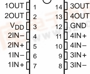
PW PACKAGE (TOP VIEW)
