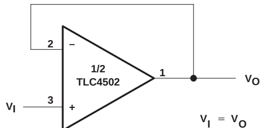
Figure 40. Voltage-Follower Circuit
