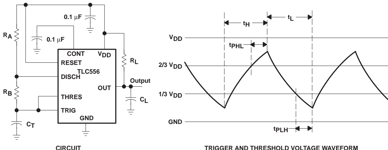
Figure 3. Astable Operation
