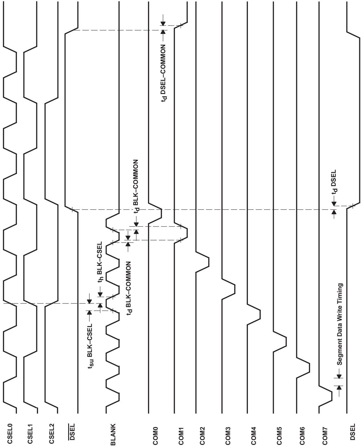
timing diagram (common driver)
