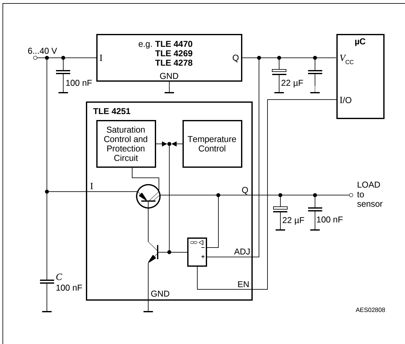
Figure 3 Application Circuit
